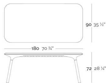
SLOO Table 180 SLOO Mesa 180
