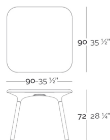
SLOO Table 90 SLOO Mesa 90
