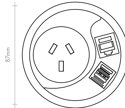
KU02: 1x GPO & 2x USB – Available in black or white
