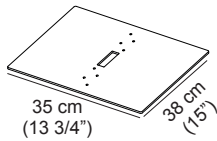
Plate single junction Art. 5109
